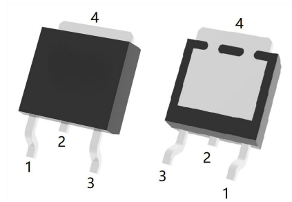
TO-252
