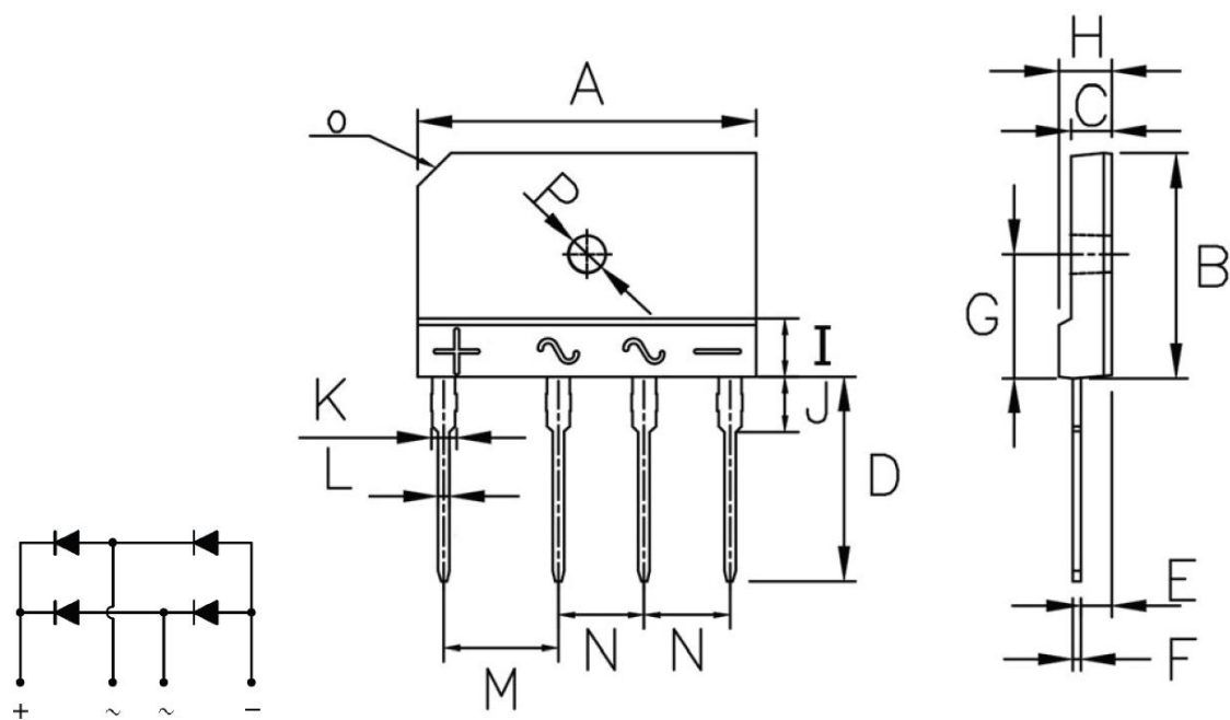
GBJ Package Outline Dimensions
