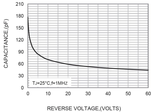
FIG.3-TYPICAL JUNCTION CAPACITANCE
