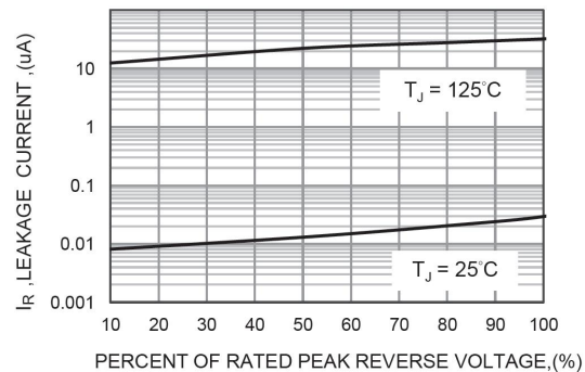
FIG.5-TYPICAL REVERSE CHARACTERISTICS
