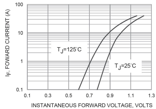
FIG.4-TYPICAL FORWARD CHARACTERISTICS
